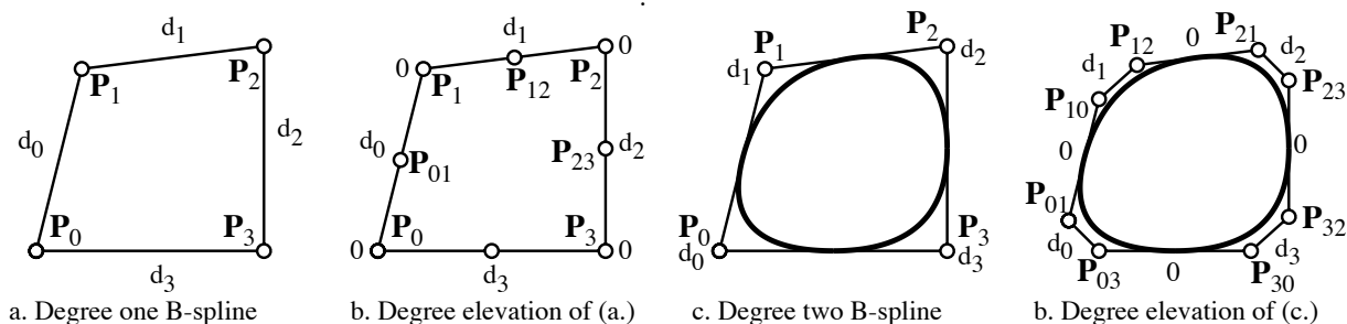
Figure 6.25: Degree elevating a degree one and degree two B-spline.
