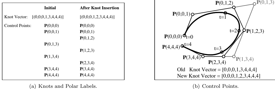
Figure 6.8: Knot Insertion.
