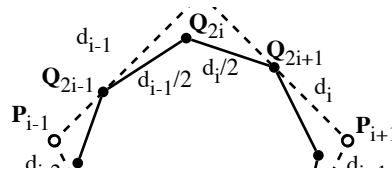
Figure 6.19: Interval halving for a non-uniform cubic B-spline curve.
