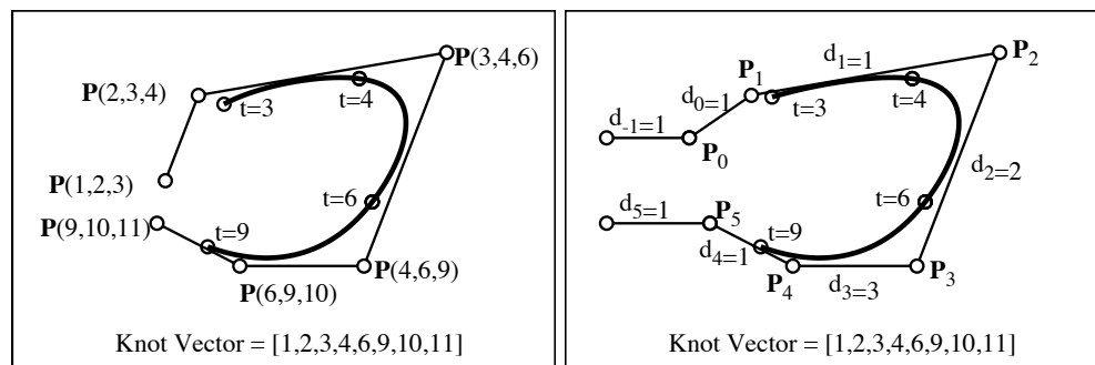
Figure 6.10: Sample cubic B-spline
