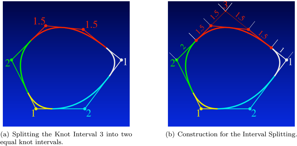
Figure 6.21: Interval Splitting of a Quadratic B-Spline Curve.
